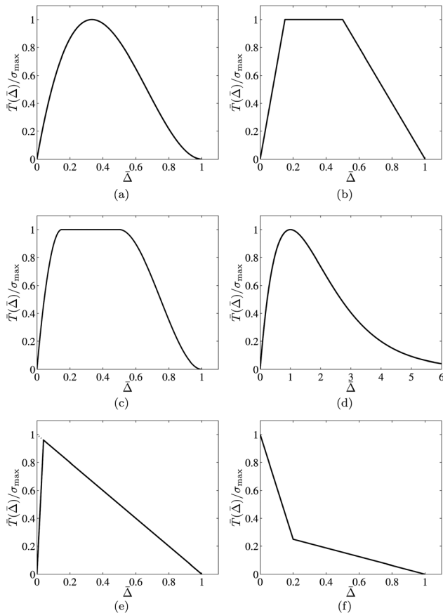
Fig. 2 Effective traction-separation relationships: (a) cubic polynomial, (b) trapezoidal, (c) smoothed trapezoidal, (d) exponential, (e) linear softening, and (f) bilinear softening
