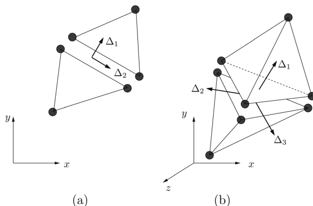
Fig. 3 Cohesive fracture separations along the local coordinate system (a) two-dimensions ( \Delta_1 , \Delta_2 ) and (b) three-dimensions ( \Delta_1 , \Delta_2 , \Delta_3 )
