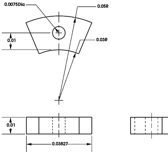
Fig. 4 Geometry of the functionally graded rotor
