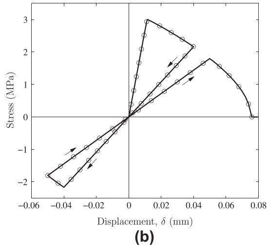
Fig. 8. Computational results: (a) mode I test, and (b) mode II test.
