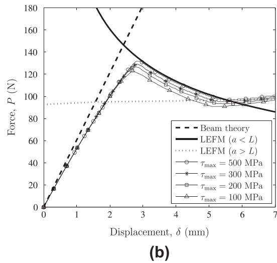
Fig. 10. Comparison between the analytical solutions and the computational results: (a) \phi_n = \phi_t = 500 N/m, and (b) \phi_n = 500 N/m, \phi_t = 1000 N/m.
