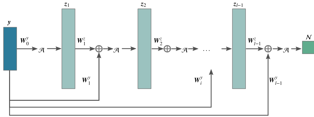
Fig. A.12. Input neural network architecture.
