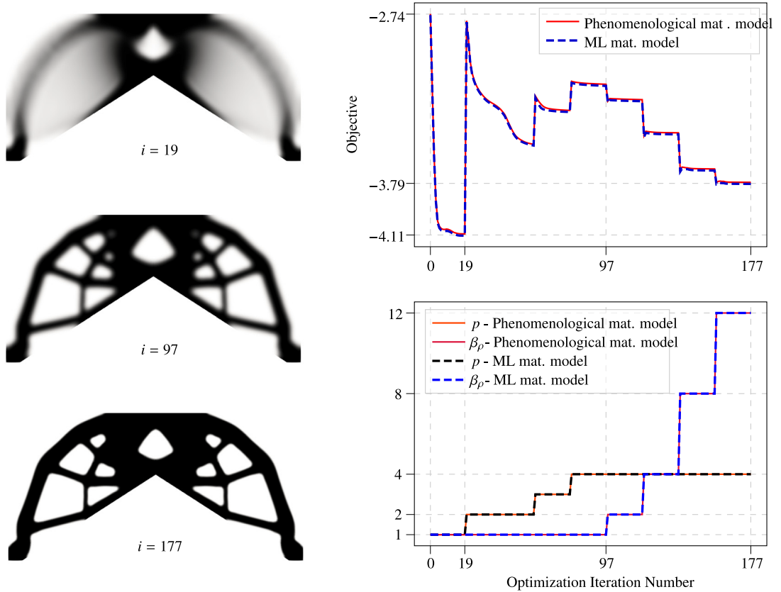
Fig. D.14. Convergence history for portal frame TO problem. Visualized designs correspond to those corresponding to TO using ML model at iterations where critical continuation parameter updates occur.
