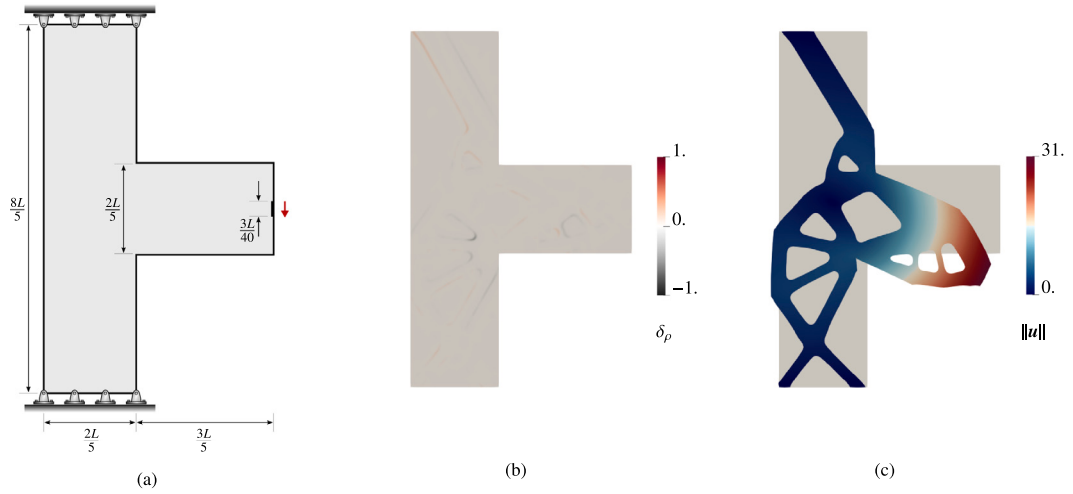
Fig. 6. (a) T-bracket boundary value problem. (b) Difference plot between the design obtained using the ML model and the design obtained using the ground truth phenomenological model, where \delta_\rho = 1 indicates material addition, and \delta_\rho = -1 indicates material removal. (c) Deformed configuration of the design obtained using the ML model.
