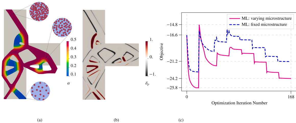
Fig. 10. (a) Deformed configuration of the final design obtained using the ML model with varying microstructure (b) Difference plot of the design obtained using the ML model with varying microstructure to the design obtained using the ML model with fixed microstructure. (c) Convergence history for the T-bracket TO problem with varying microstructure versus fixed microstructure.
