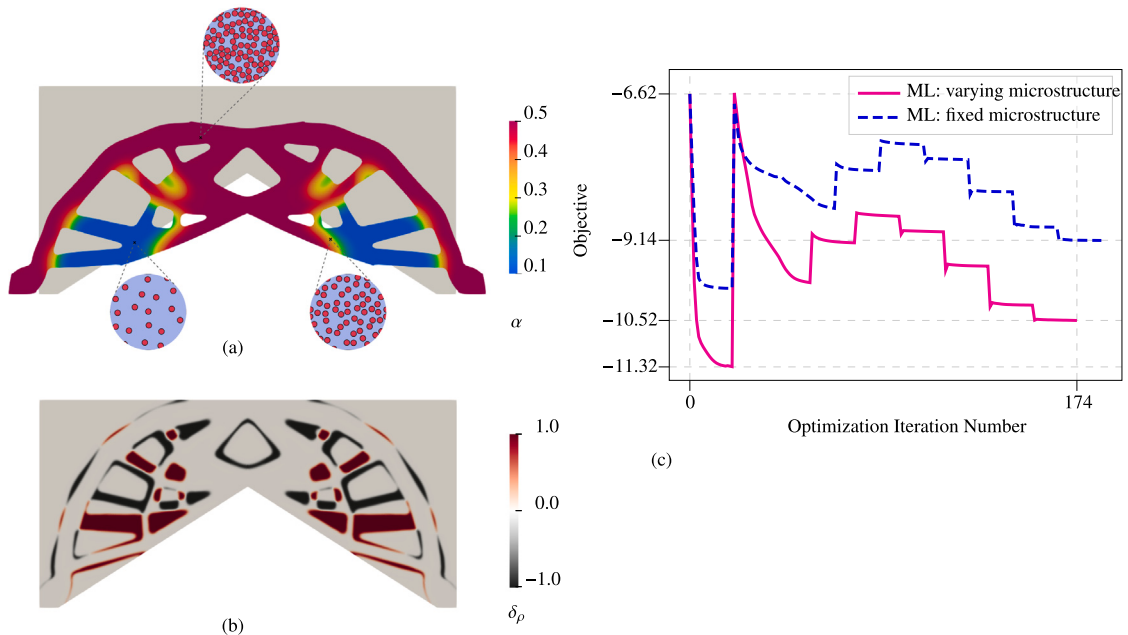
Fig. D.15. (a) Deformed configuration of the final design obtained using the ML model with varying microstructure (b) Difference plot between the design obtained with varying microstructure and the design obtained with fixed microstructure. (c) Convergence history for the portal frame TO problem with varying microstructure vs. fixed microstructure.
