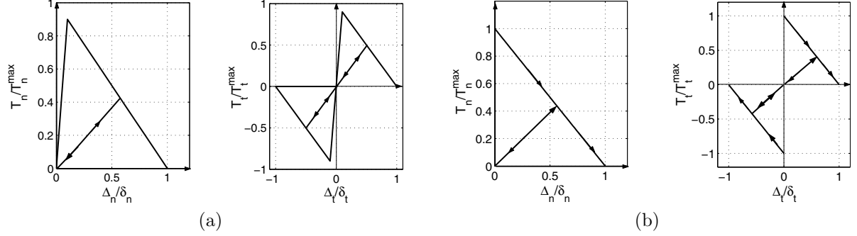
Fig. 2: Comparison of two typical intrinsic and extrinsic CZMs: (a) bilinear intrinsic cohesive zone model [5] in pure tension and pure shear, respectively; (b) initially-rigid extrinsic cohesive zone model [4] in pure tension and pure shear, respectively.
